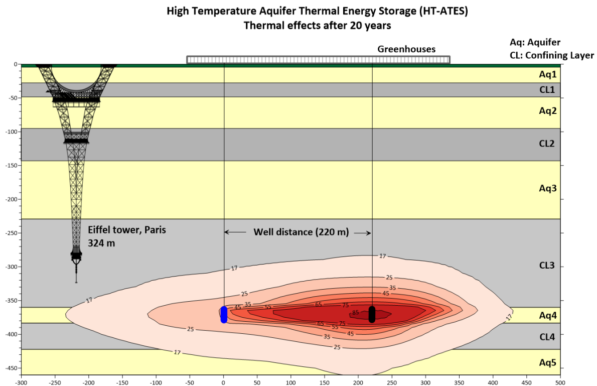
Figure 3: Simulated temperatures ( ^\circ\text{C} ) in the subsurface after heat storage in year 20 for a worst-case scenario. The heat is stored in a 23 m thick sand layer that is located deeper than the height of the Eiffel tower. A thick clay layer overlies the storage aquifer and prevents significant heat losses to shallower aquifers. The relative cold well (blue) and hot well (black) are indicated with thick lines which are not to scale.
