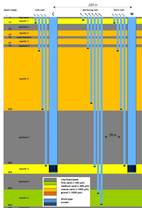
Figure 2: Schematic cross-section through the subsurface at the wells (not to scale). Coarse/medium coarse and fine sands in orange/yellow/green. Clay layers in grey. Blind pipes of the wells and piezometers indicated in blue, well/piezometer screens hatched black. Aquifer 4 is the storage aquifer.
